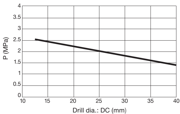
Coolant pressure
